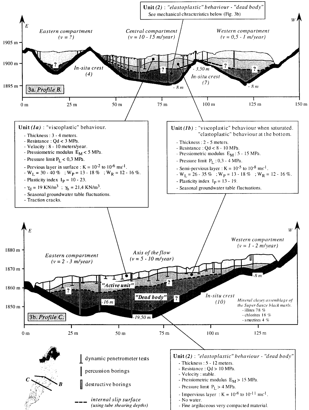
Fig. 3. Internal structure, mechanical and hydrodynamical characteristics of the flow (3a. B cross-section , 3b. C cross-section). (Genet et Malet, 1997, Herrmann, 1997, Klotz, 1998).
