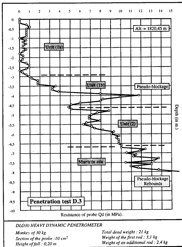
Fig. 2. Penetrometric curve D.3.
