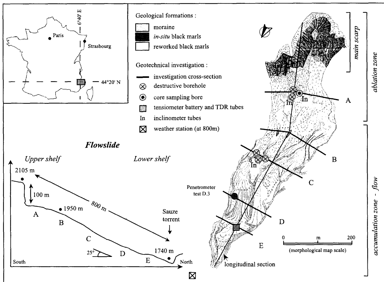
Fig. 1. Geographic setting of the earthflow and of the investigation cross-sections.
